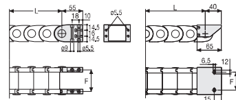
Fig. B Chain fixed outside the radius. (Fig. B) See end brackets mounting variations page 51.
