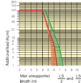
Fig. A Chain fixed outside or inside the radius, (Fig. A)
